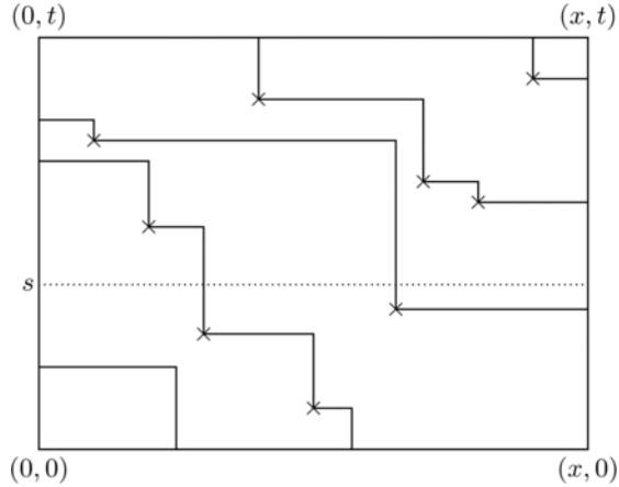
FIG. 1. Space-time paths of the Hammersley's process, with sources and sinks.
